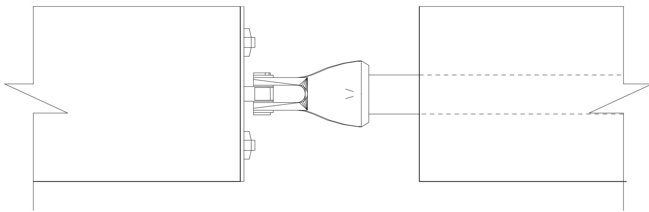
SLAB + WIND NEEDLE DETAIL | SCALE: 1/8" = 1'-0"
