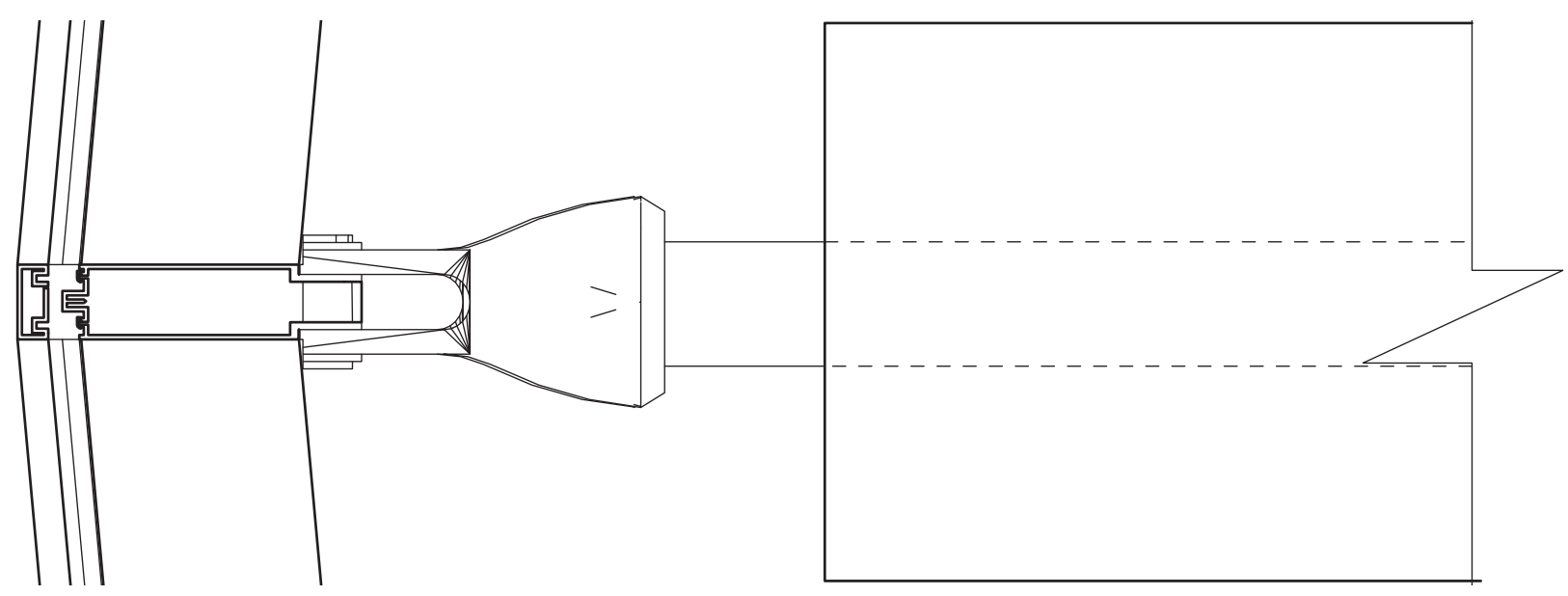
MULLION + WIND NEEDLE DETAIL | SCALE: 1/8" = 1'-0"
